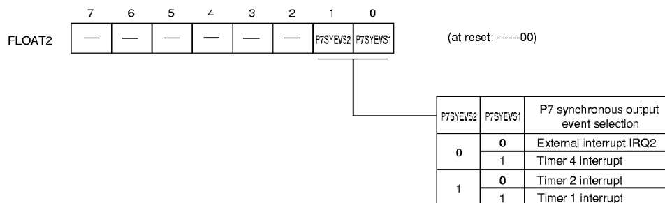
Figure 3-2-5 Pin Control Register 2 (FLOAT2: X'03F4C', R/W)
